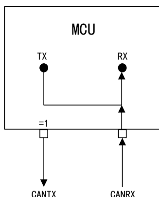
Figure 105 CAN Works in Silent Mode
